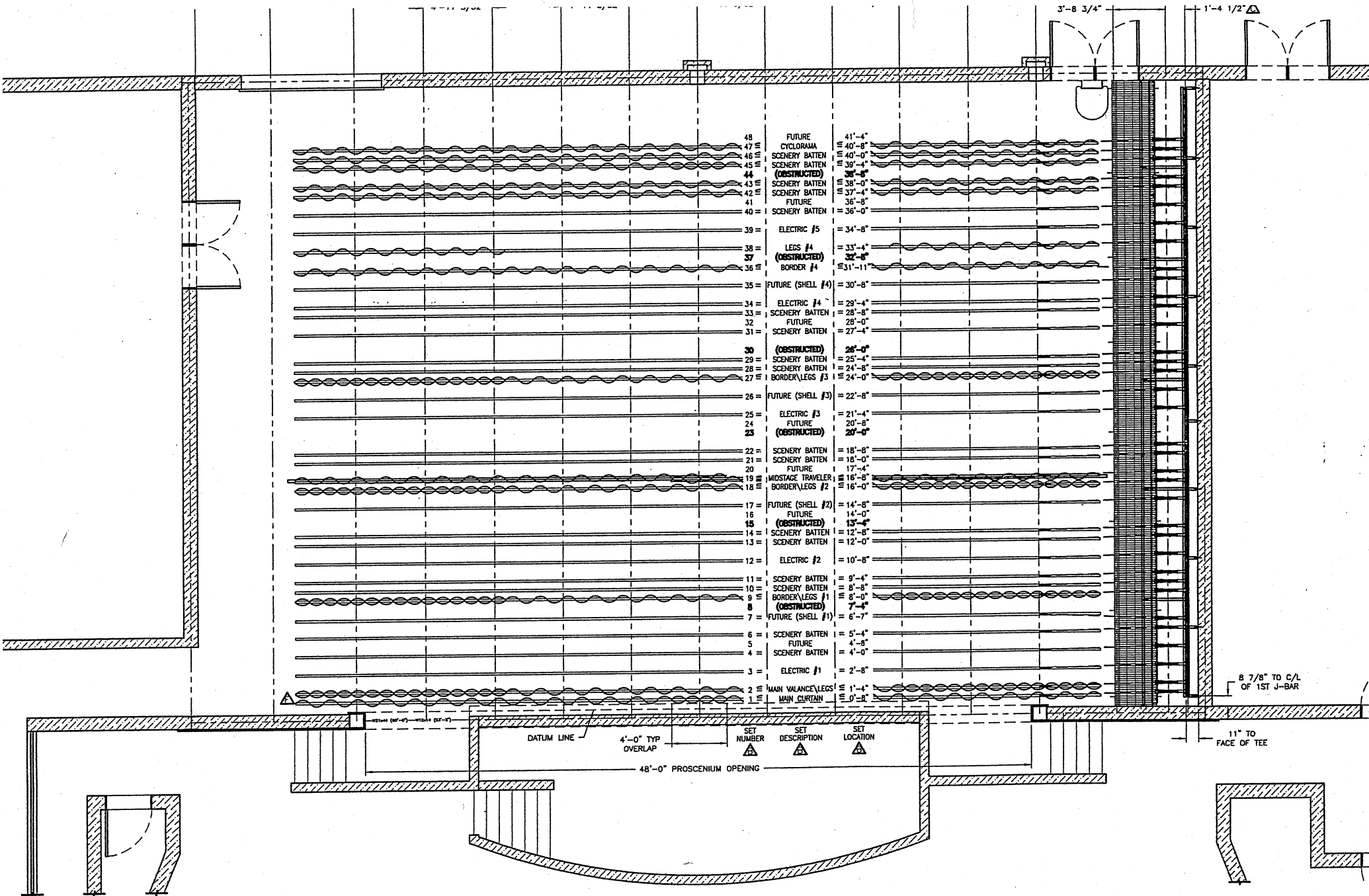
PLAN VIEW - STAGE EQUIPMENT SCALE: 1/4" = 1'-0"
